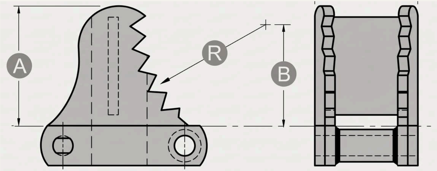
SLASHER FLIGHT DIMENSIONS
