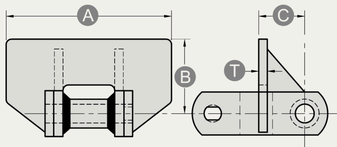
RF12 ATTACHMENT
