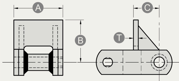
RF2 ATTACHMENT
