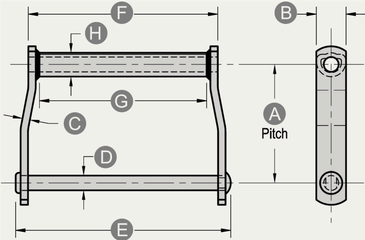
"SUPER" DRAG CHAIN DIMENSIONS
