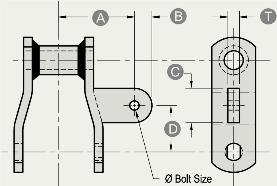
A22 ATTACHMENT
