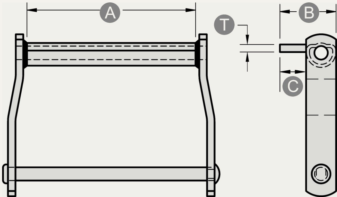
"C" ATTACHMENT DIMENSIONS
