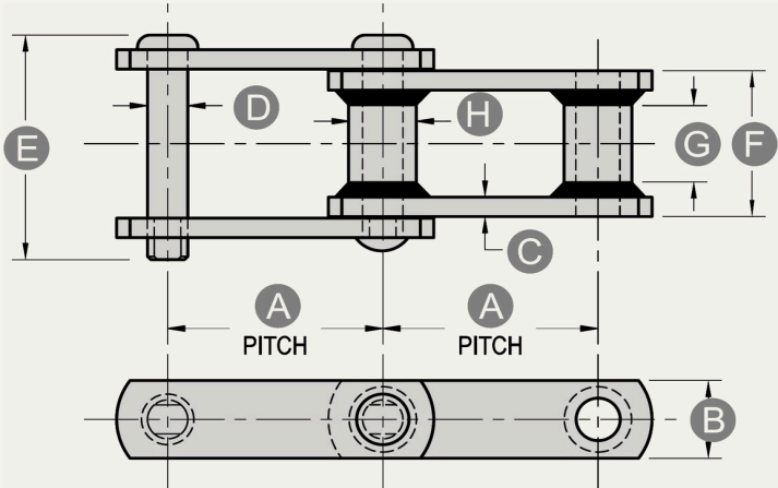
WRC STRAIGHT SIDEBAR CHAIN DIMENSIONS
