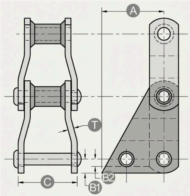
S1/S2 ATTACHMENT DIMENSIONS
