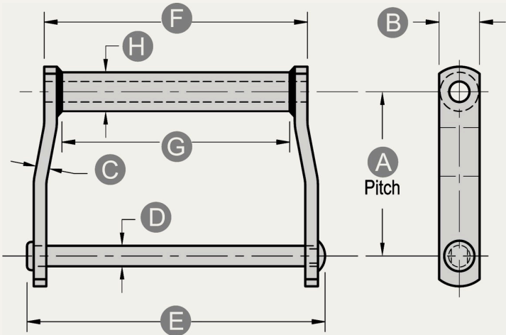
"MEGA" DRAG CHAIN DIMENSIONS
