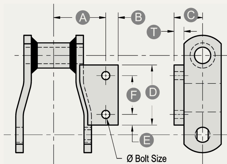
A2 ATTACHMENT
