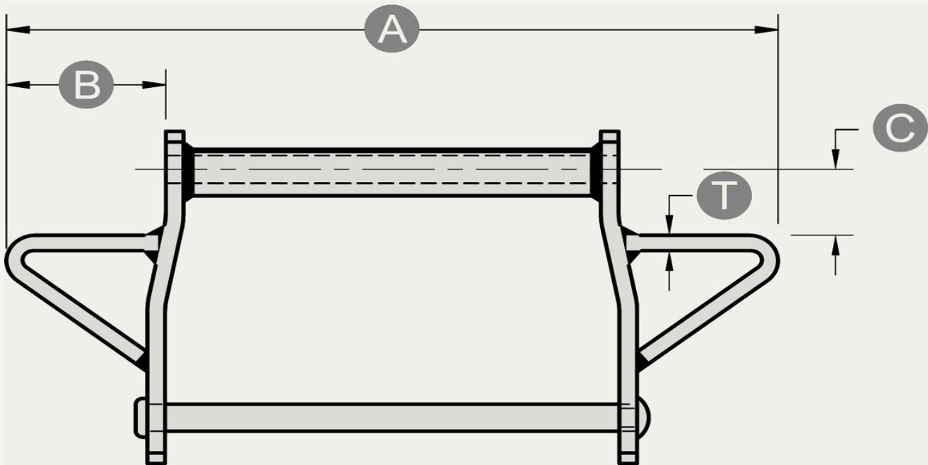
STANDARD WING ATTACHMENT DIMENSIONS
