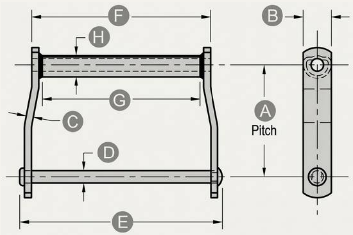
WD CHAIN DIMENSIONS
