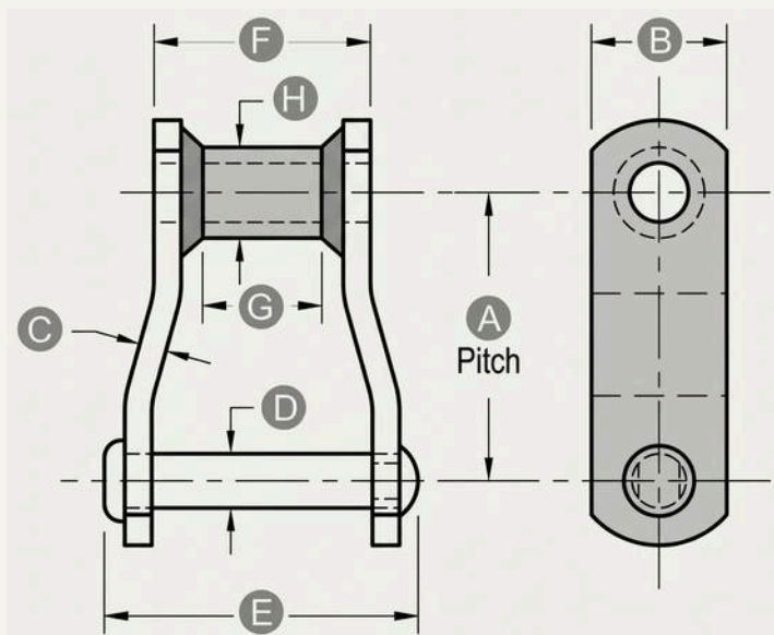
WR OFFSET SIDEBAR CHAIN DIMENSIONS
