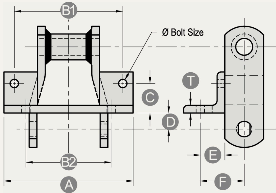
F2/F4 ATTACHMENT
