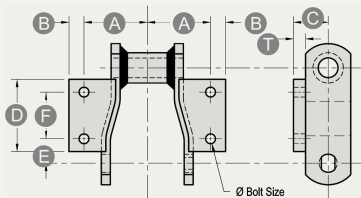
K2 ATTACHMENT
