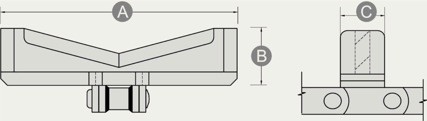
BEVELLED V-FLIGHT DIMENSIONS
