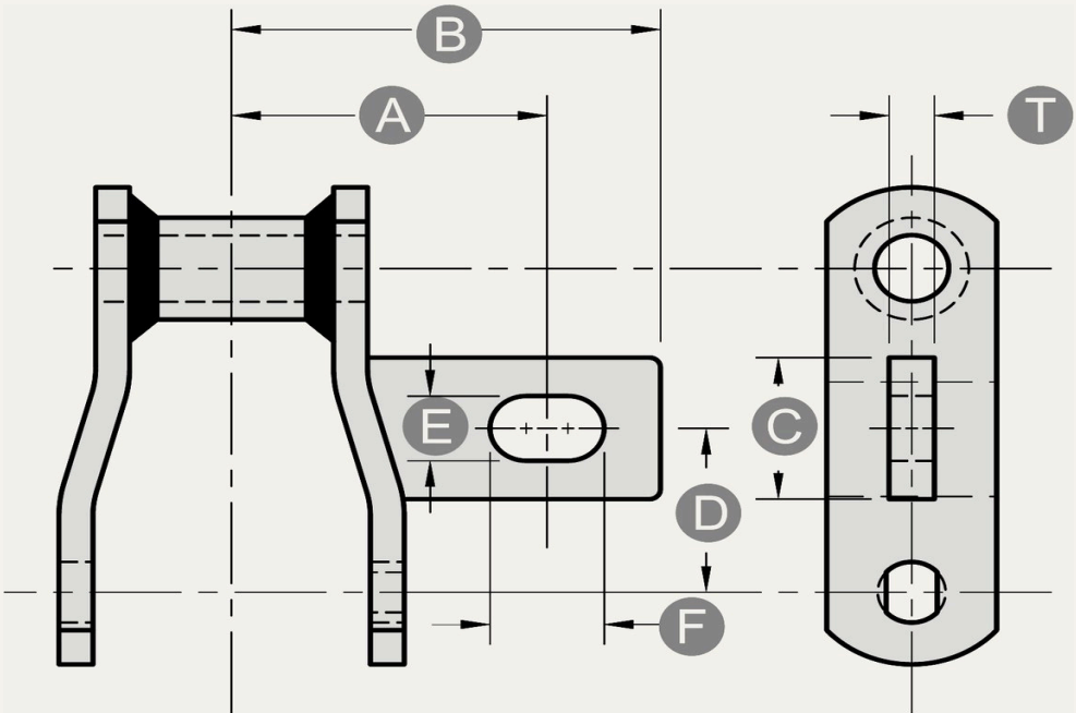
SLOTTED A22 ATTACHMENT
